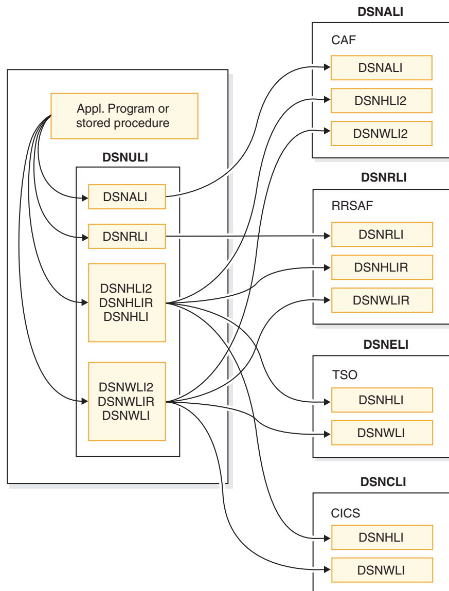
Figure 4. Application program or stored procedure linked with DSNULI
