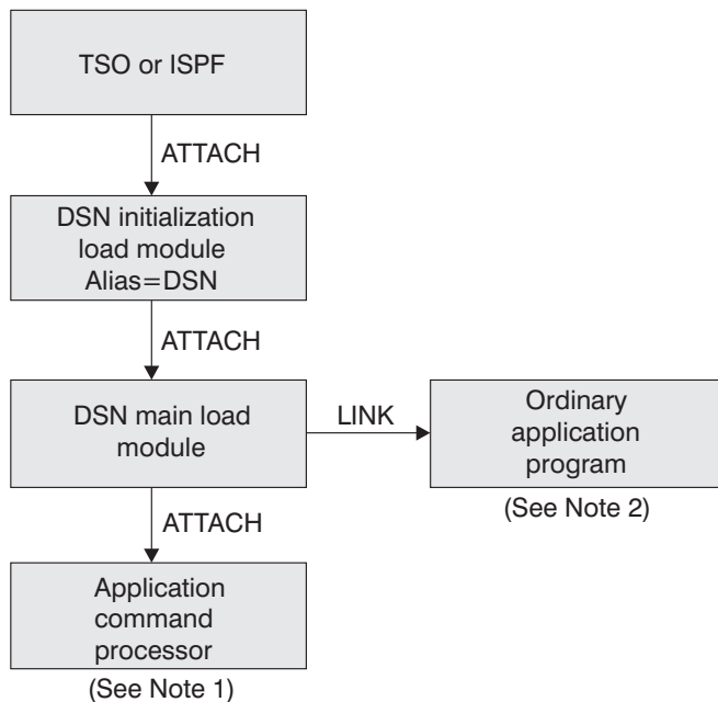
Figure 80. DSN task structure
