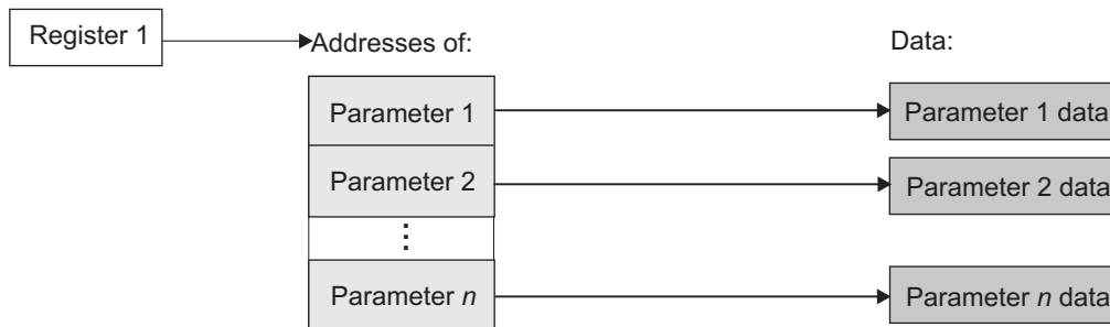
Figure 33. Parameter convention GENERAL for a stored procedure
