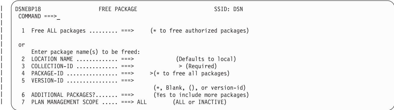
Figure 77. The Free Package panel
