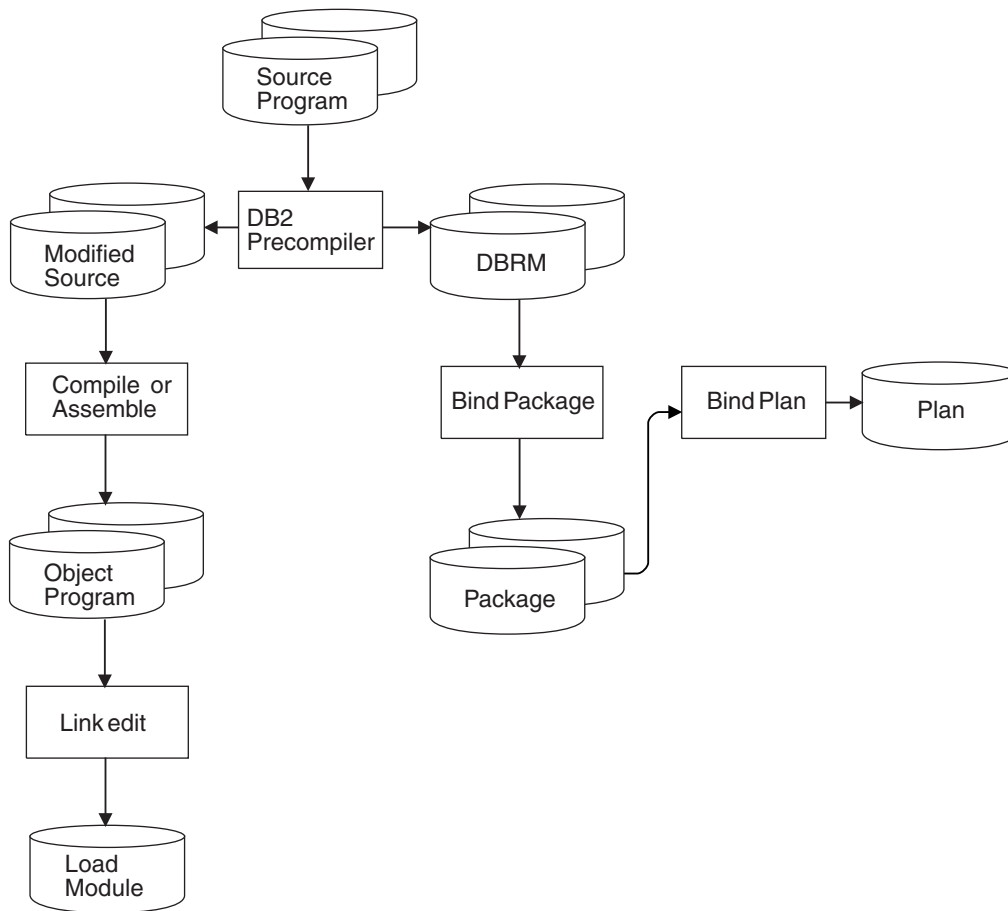
Figure 58. Program preparation with the DB2 precompiler
